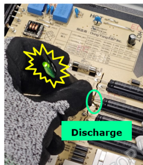
Before Discharging
