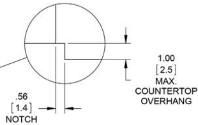
TYPICAL ISLAND INSTALLATION (AGB122 SHOWN)
