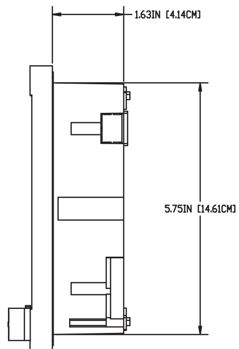
Side View with Bezel (above)
