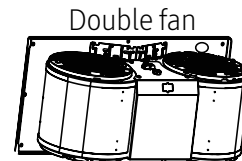
Motor fan assembly 30" (Single fan) 36" (Double fan) 48" (Double fan)
