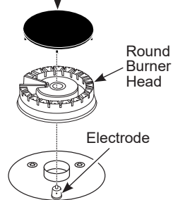
Round Burner
