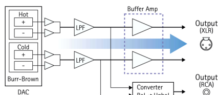
Balanced Circuit (CD-S2000)
