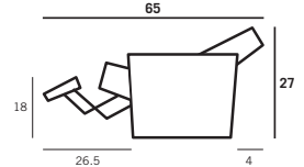
Side View (wall saver mechanism, fully reclined)
