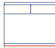
ARMLESS LOVESEAT
