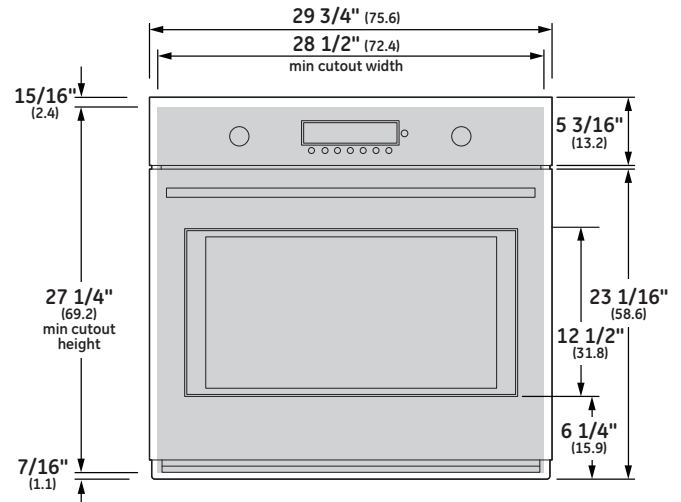
FRONT VIEW (SHOWING CUTOUT OVERLAP)
