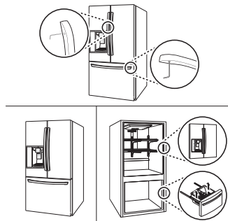
Disassembling/Assembling
