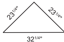
TOP VIEW 73230, 73235 73272, 73275
