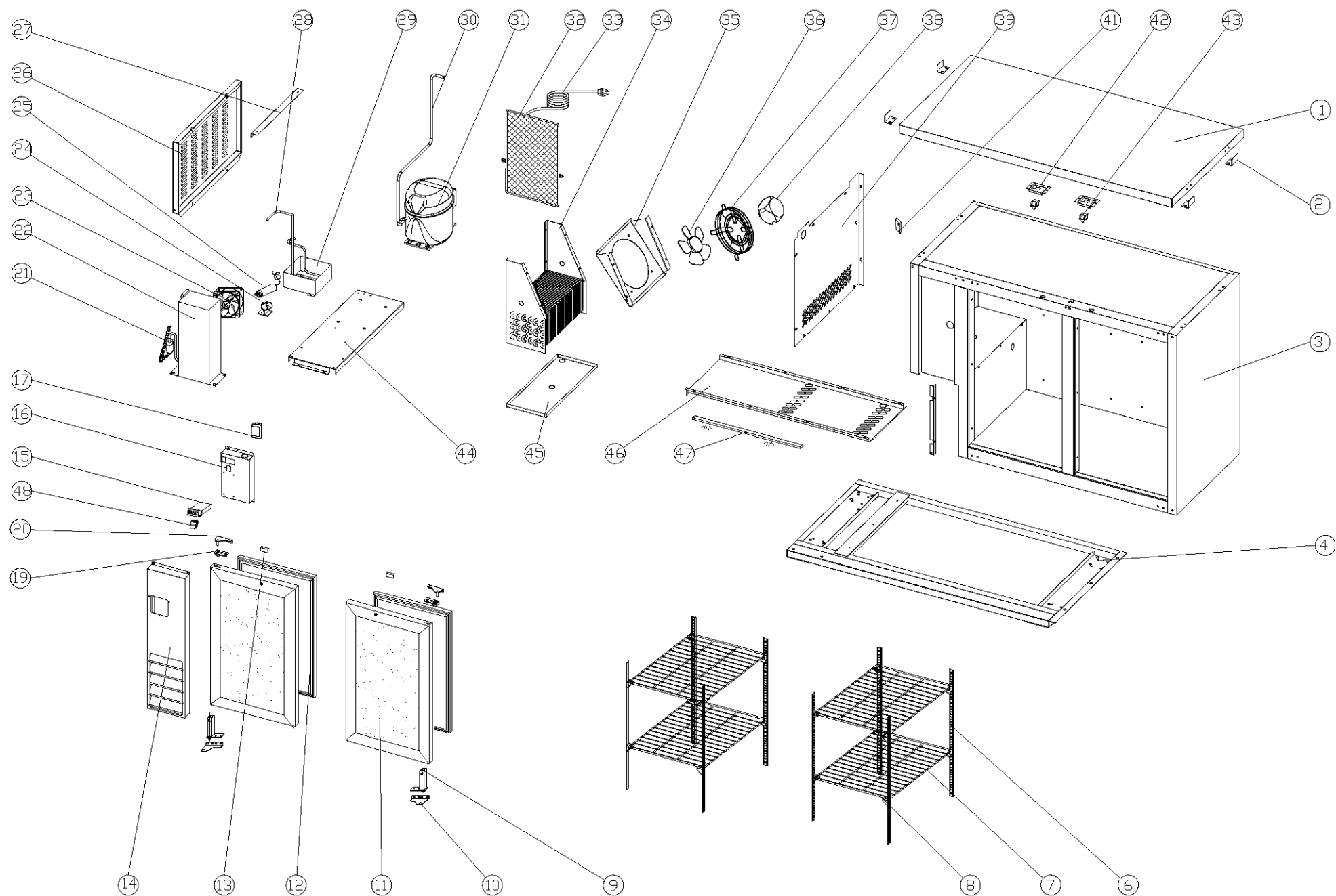
KELVINATOR COMERCIAL KCHBB60G - exploded view
