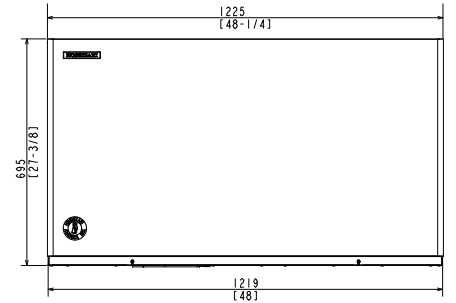
REMOTE AIR-COOLED
