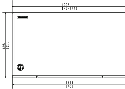
WATER-COOLED
