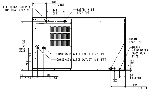
WATER-COOLED
