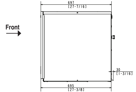
REMOTE AIR-COOLED
