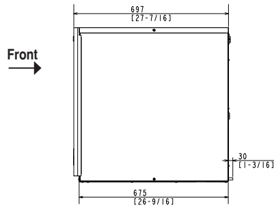
WATER-COOLED
