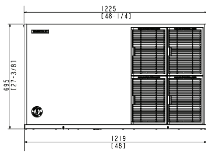
AIR-COOLED
