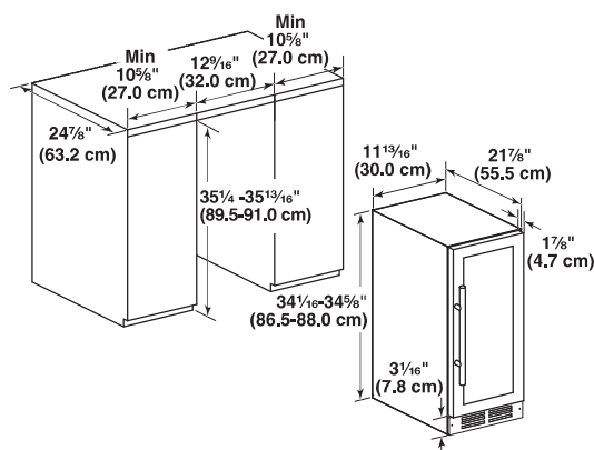
Critical dimensions for 15" models
