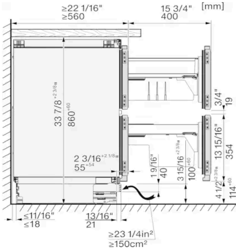
KU7175D, Built-under, side view
