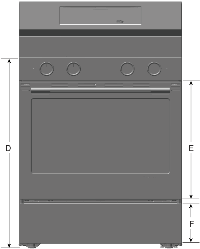
VISTA FRONTAL
