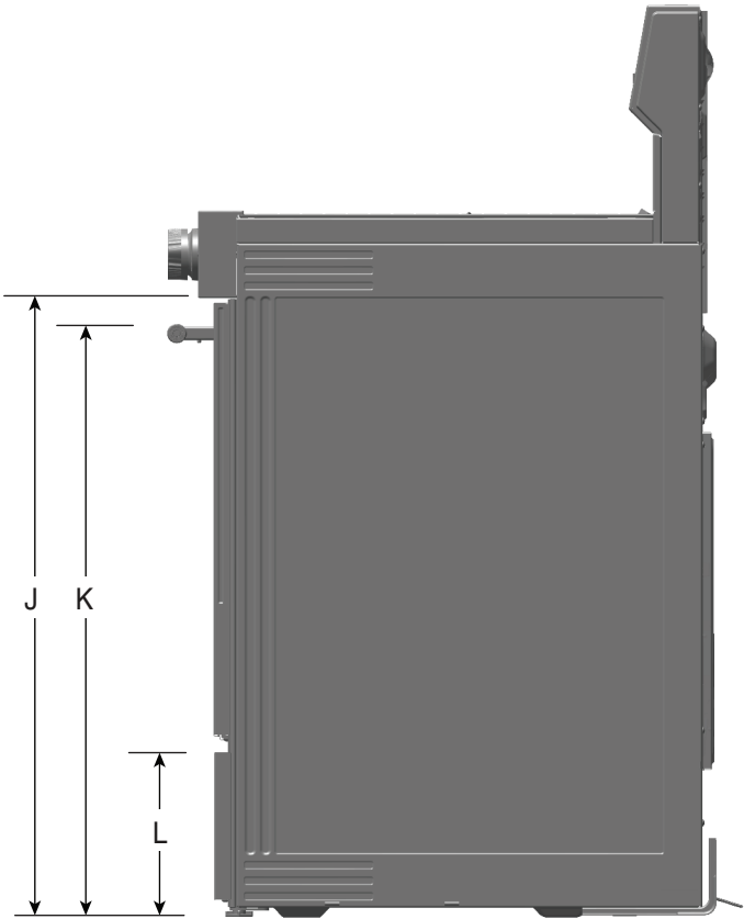
SIDE VIEW
