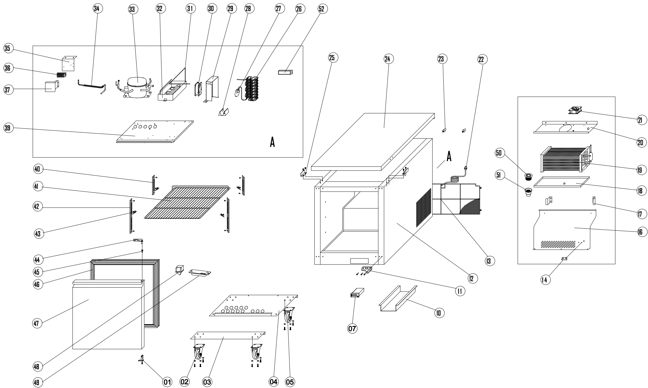
EXPLODE OF KCHUC27R
