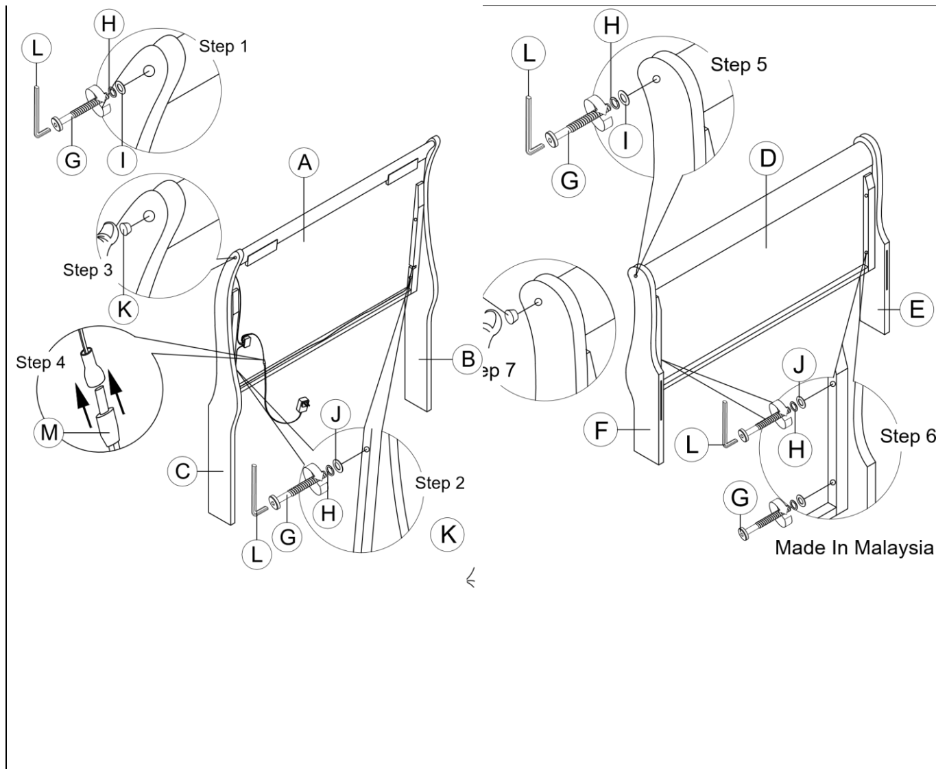
CHARLIE TWIN HEADBOARD WITH LED / FOOTBOARD
