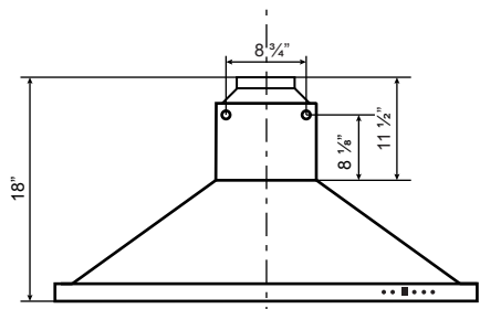
FRONT WITHOUT FLUE
