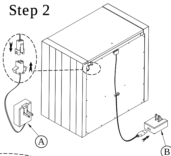
Tool Required (not provided) Phillips Screwdriver
