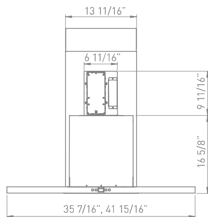
FRONT
