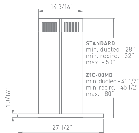
SIDE
