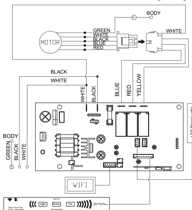
External/In-Line Blower Wiring Diagram
