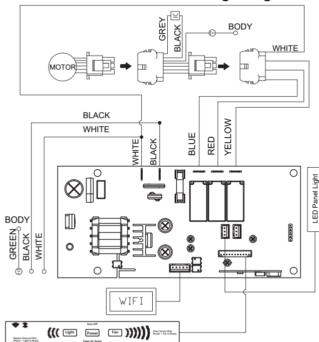
Internal Blower Wiring Diagram
