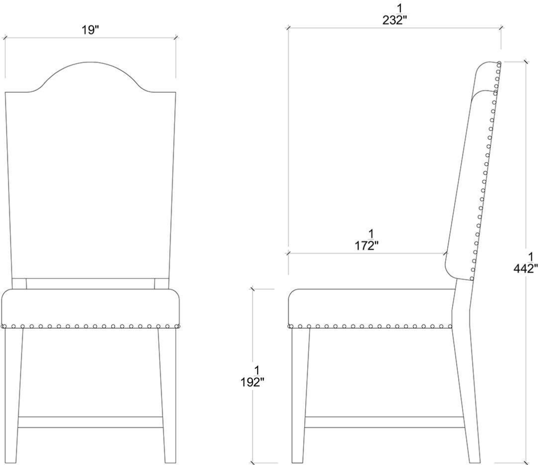
FRONT VIEW
