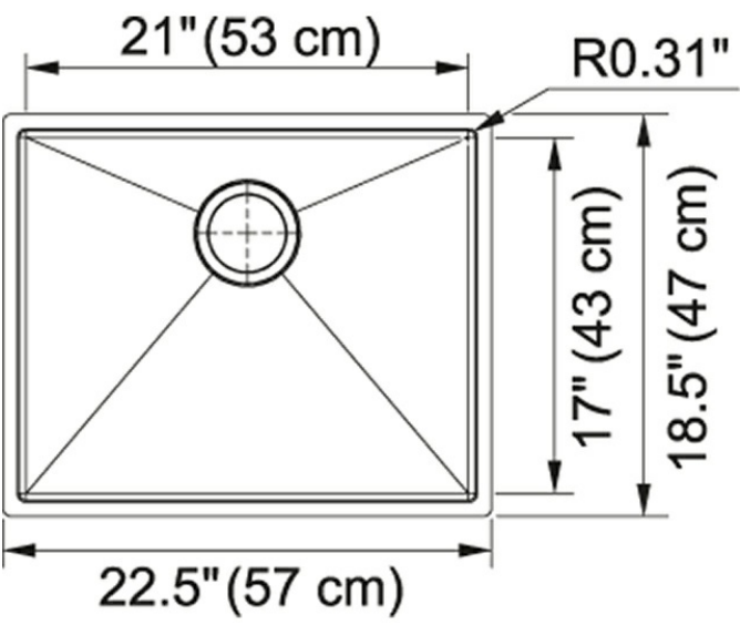
Technical Drawing
