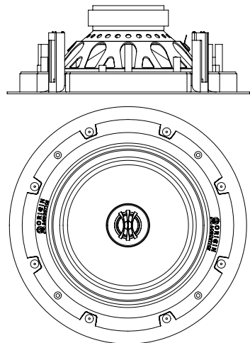
Figure 2.1: Speaker Side and Front View
