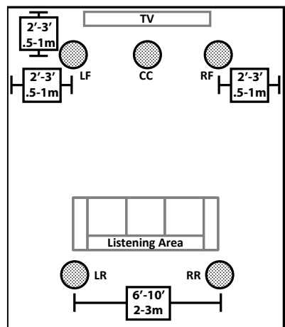
Figure 3.3: 5 Speaker Setup
