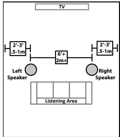
Figure 3.2: 2 Speaker Setup
