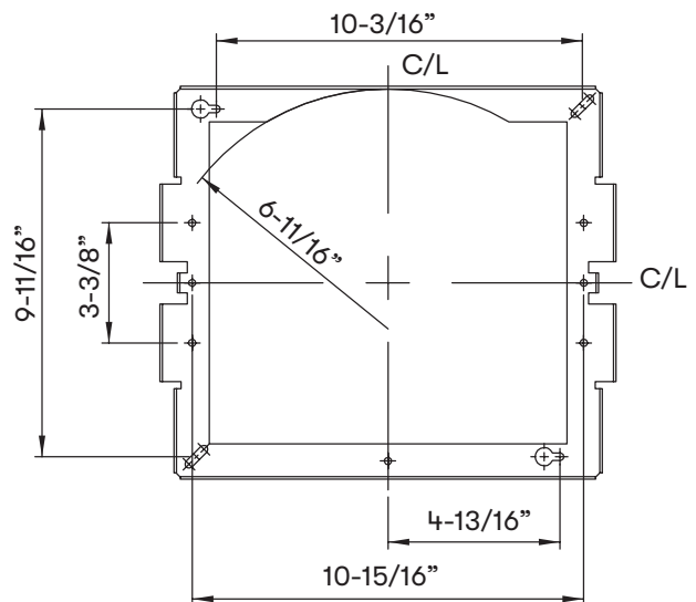
Top Support Frame (top view)
