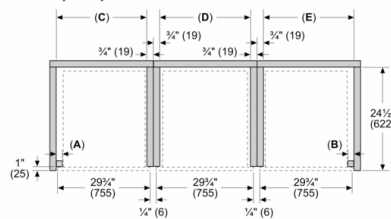
Flush side-by-side-by-side installation
