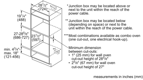
Standard installation 30" speed oven or microwave above a single oven***
