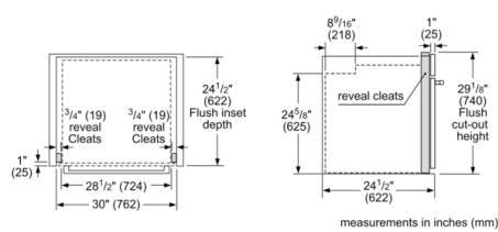
Flush installation Top view
