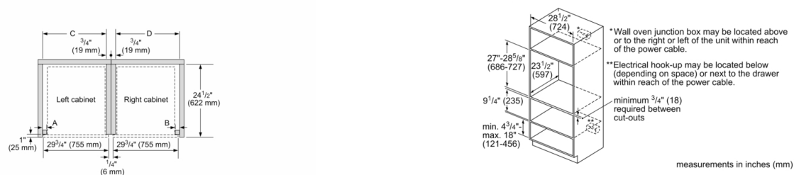
Standard installation 30" single oven over storage or warming drawer
