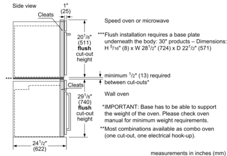
Flush installation Speed oven or microwave above a 30" single oven**
