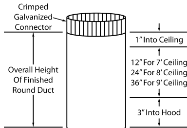
Finished Round Duct
