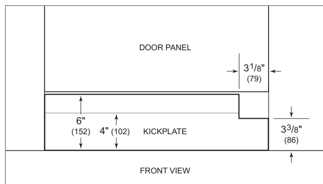
Kickplate notch
