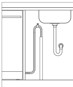
Tubo vertical
