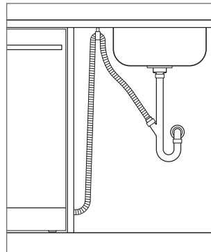
High loop to P-trap
