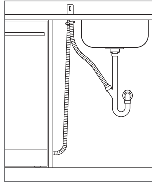
Air gap to P-trap
