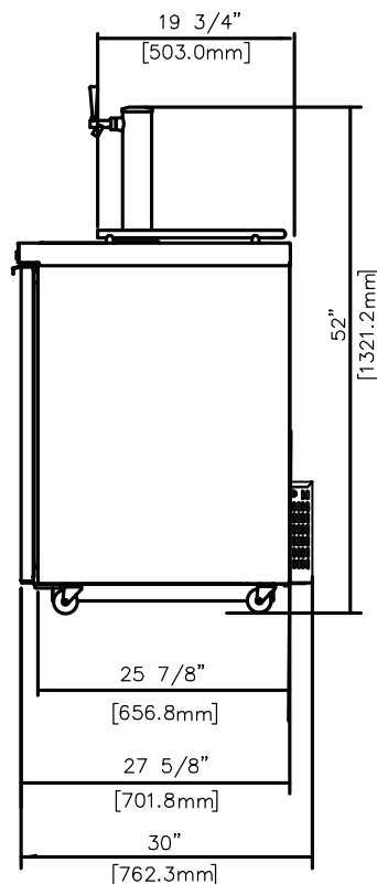
DD24(-S) Side View
