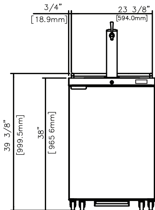
DD24(-S) Front View
