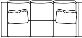
560-0113 3-over-3 Sofa 85 W 38 D 35 H 29 AH 21 SH
