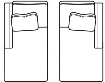
560-087 LSF Chaise 560-085 RSF Chaise 35 W 65 D 35 H 29 AH 21 SH
