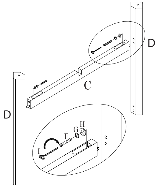
ASSEMBLY BOTTOM CROSS STRETCHER(C )
