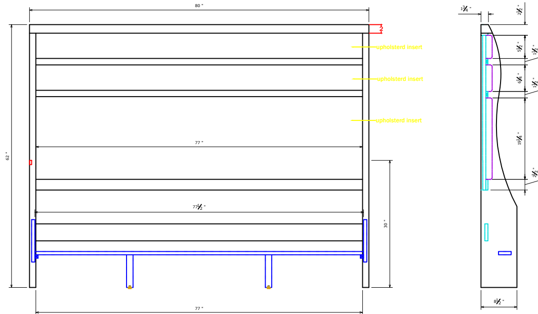
ZARC-7104 Arcadia King Sleigh HB
