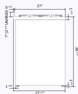
Side view UM30
