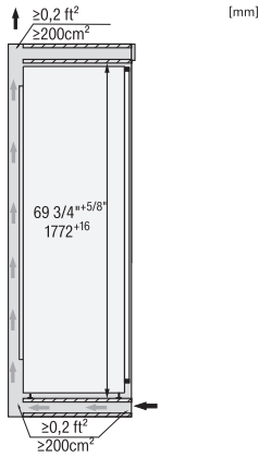
KS7793D, FNS7794E, side view (installation drawings) (US)
