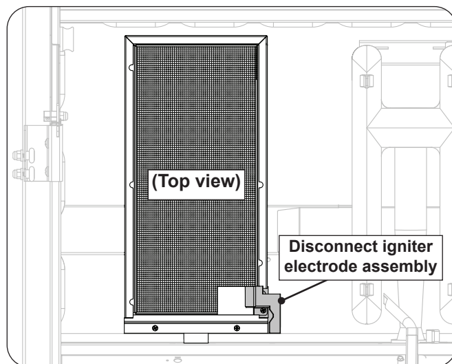
Fig. 48-4 Infrared burner removal
