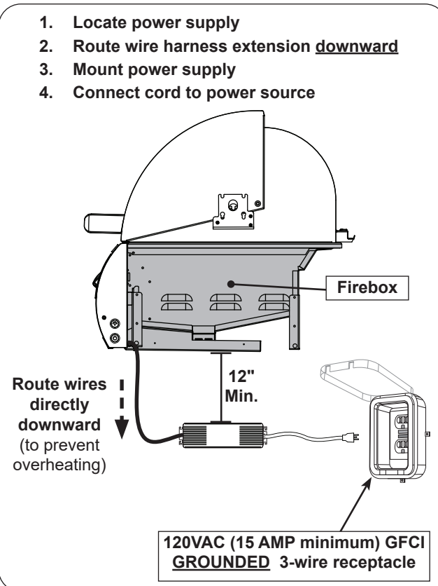
Fig. 29-3 Electrical installation
