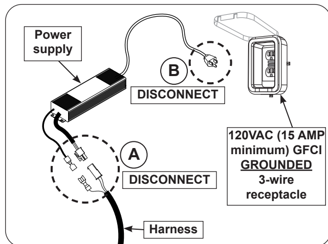
Fig. 48-1 Perform system reset
