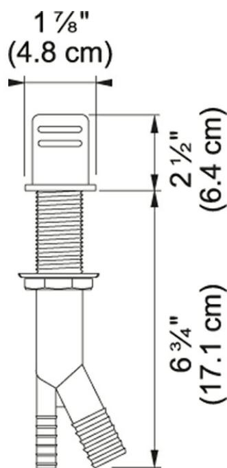
Technical Drawing
