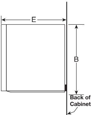
SIDE VIEW 2
