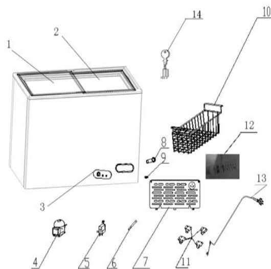
Explosion View Of KCNF073WS
