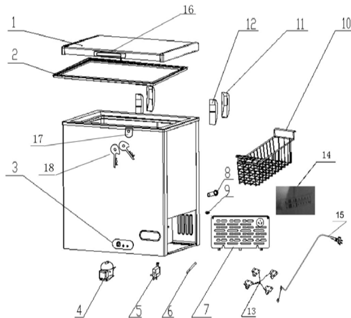
Explosion View Of KCCF073WS
