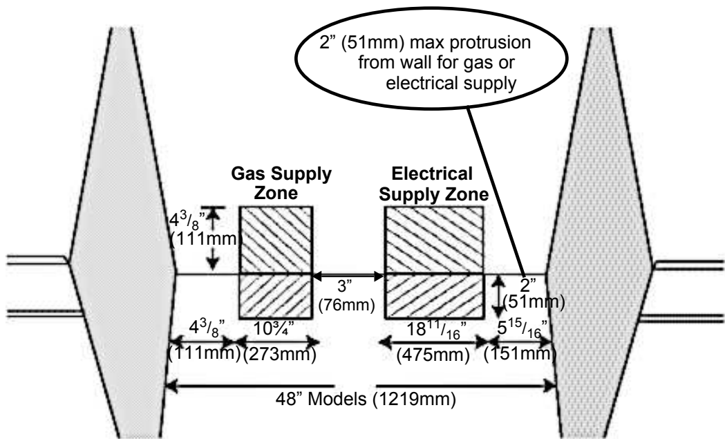
Gas & Electrical Supply Locations for 48" Dual Fuel Ranges
