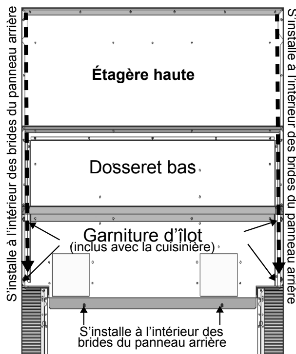
Figure 22 : Installation du dossier
