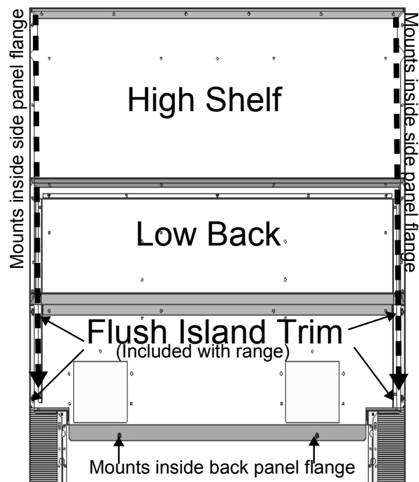
Figure 22: Backguard Installation
