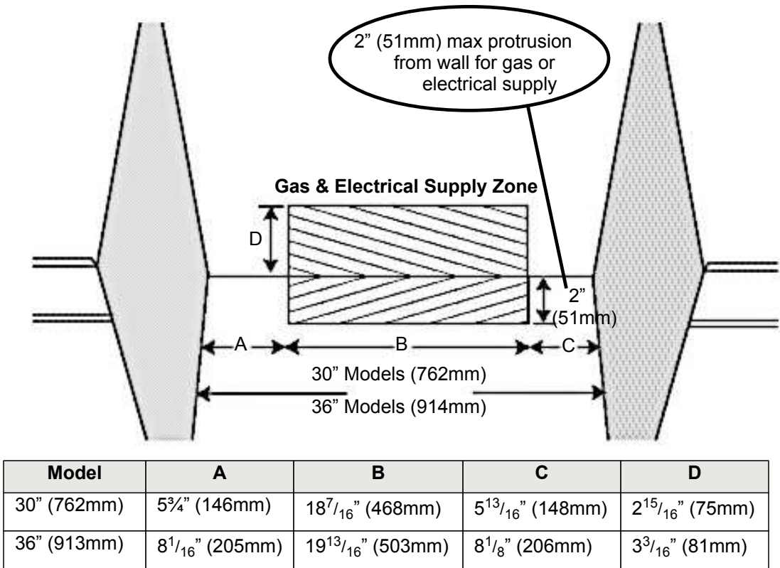
Gas & Electrical Supply Locations for 30" and 36" Dual Fuel Ranges
