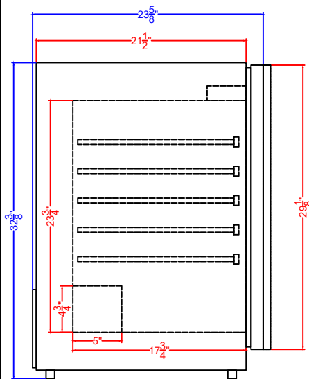
Panel Dimensions See manual for exact installation instructions
