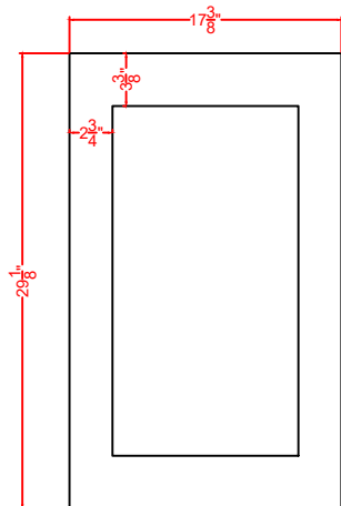
Panel Dimensions See manual for exact installation instructions
