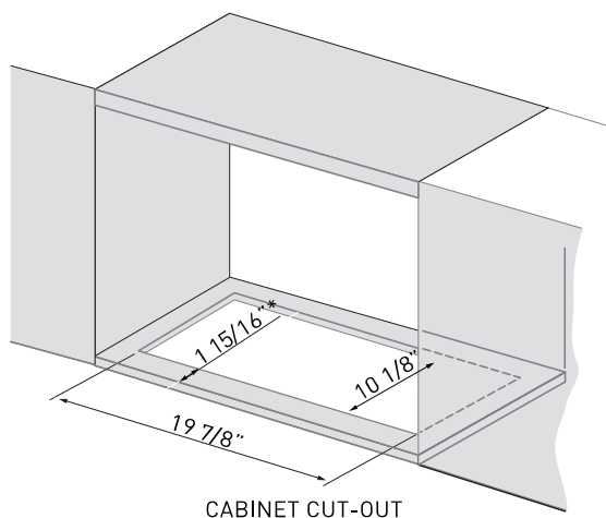
CABINET CUT-OUT
