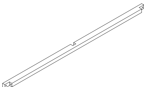
(E) Front- Middle Rail (x2)
