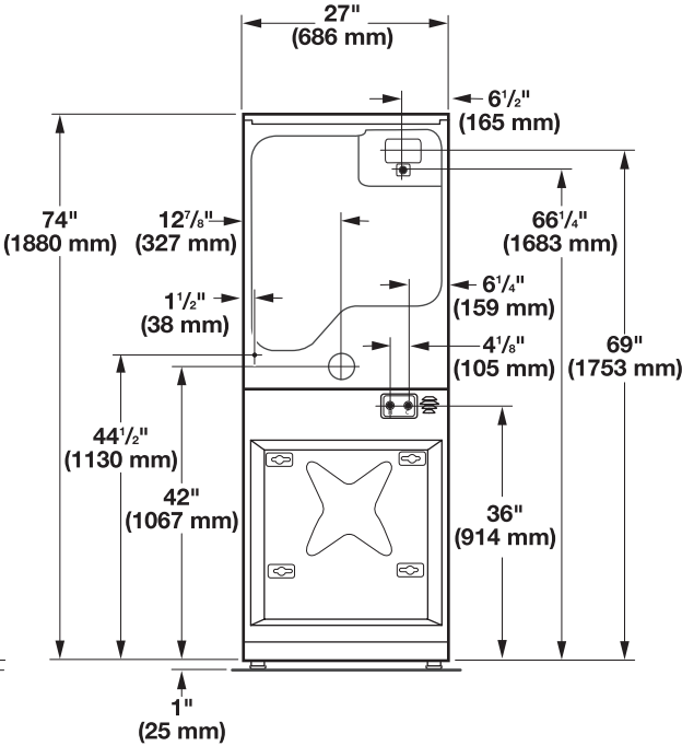
Back View
