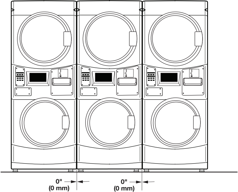
Side Clearances
