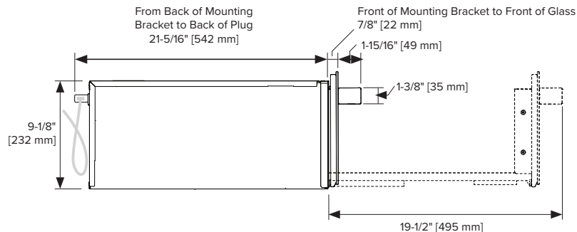
SIDE
