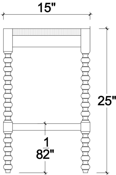
FRONT/SIDE VIEW
