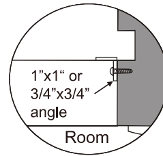
FIG.20C Add 16- or 18- gage angle
