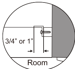
FIG.20A Add angle to wood stop
