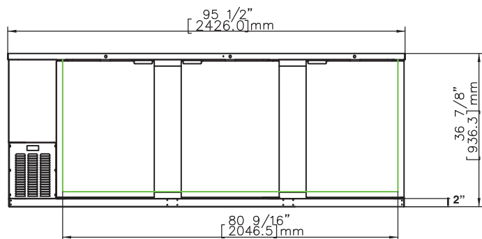
BB95(-S) Front View
