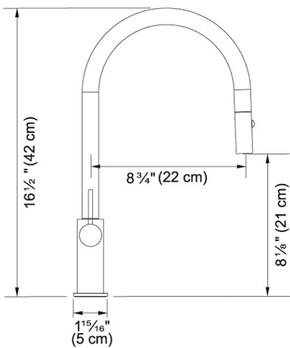
Technical Drawing
