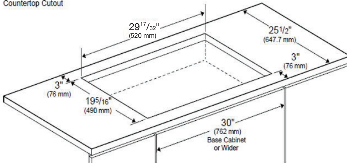
Countertop Cutout
